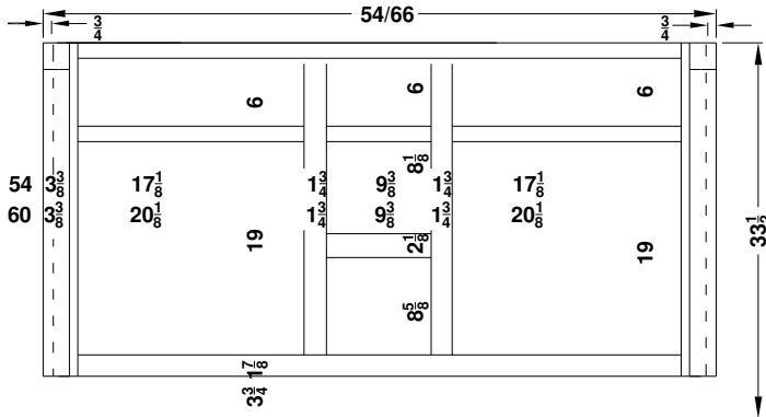
BD5421M/18M BD6021M/18M
